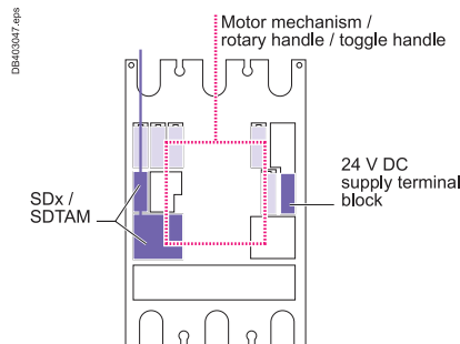
Remote indications via SDx or SDTAM
