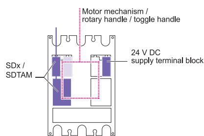
Remote indications via SDx or SDTAM
