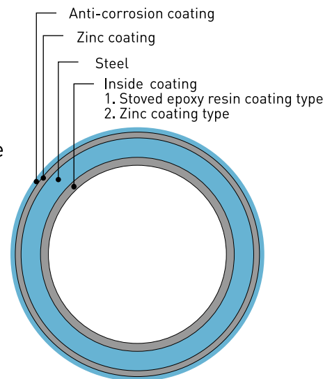
CROSS-SECTIONAL VIEW OF Panasonic WHITE CONDUIT
