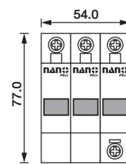
3 Pole 10-20 kA
