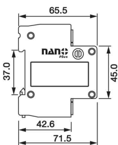
1 Pole 20-40 kA
