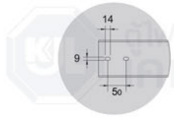
SIDE
